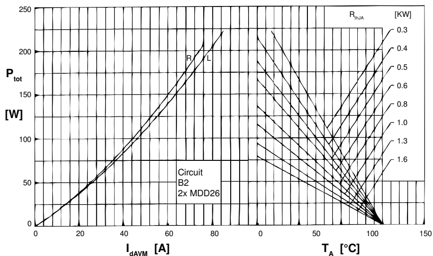
Fig. 6 Single phase rectifier bridge: Power dissipation vs. direct output current I and ambient temperature; R = resistive load, L = inductive load
