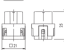
Гнездо EBM05CP00 Female Insert
