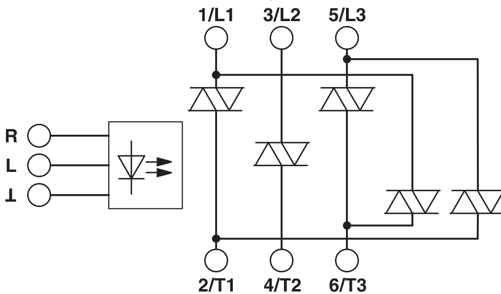
Block diagram
