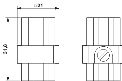
Dimensioned drawing
